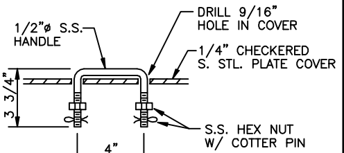
HANDLE DETAIL
