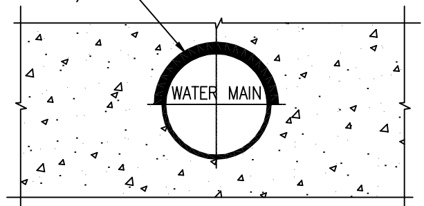
FILLER DETAIL
